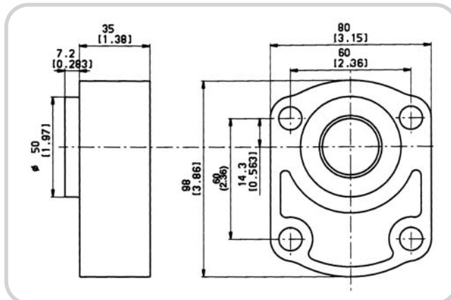
code CL With shaft code 25, 26
