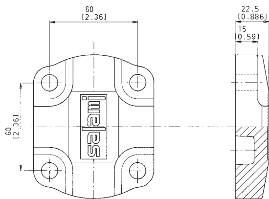
Standard rear cover for unidirectional pumps
