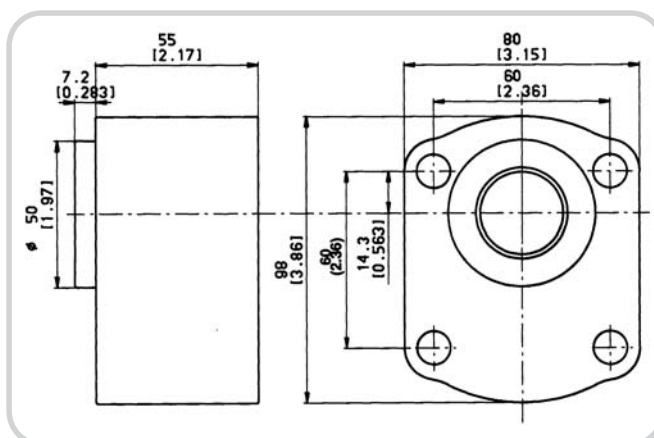
code CF With shaft code 25, 26
