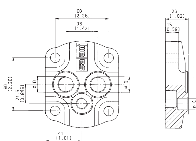
For motors with threaded rear ports until 22 l/min delivery.
